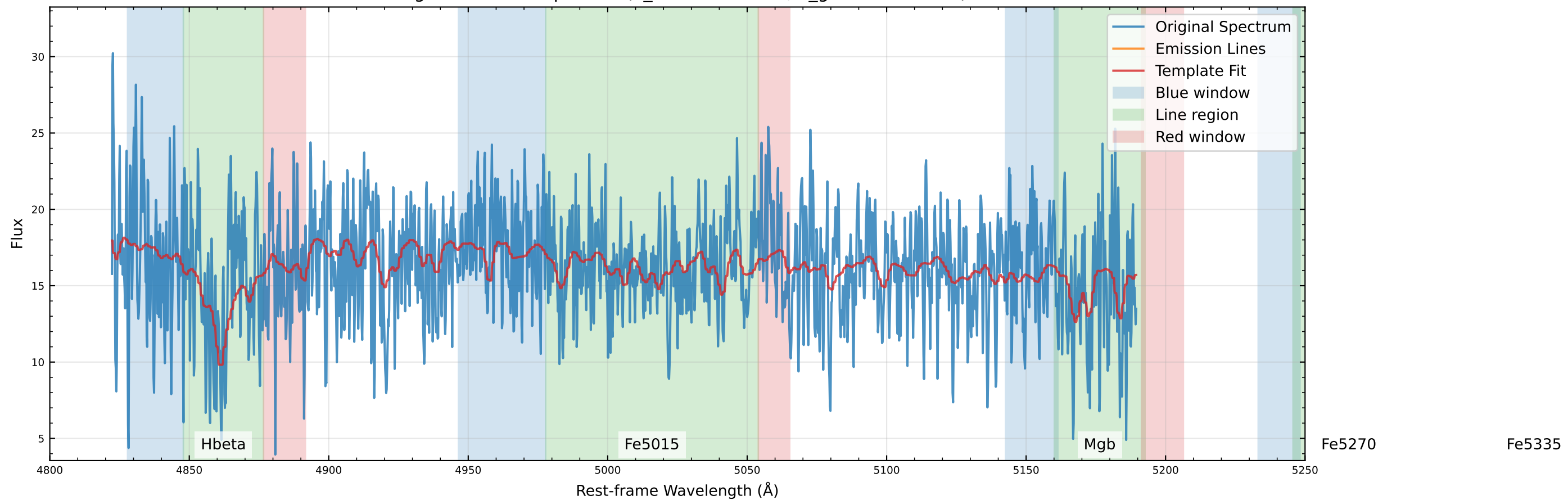
Original Data Comparison (v_star=-6.7 km/s, v_gas=-48.1 km/s)
