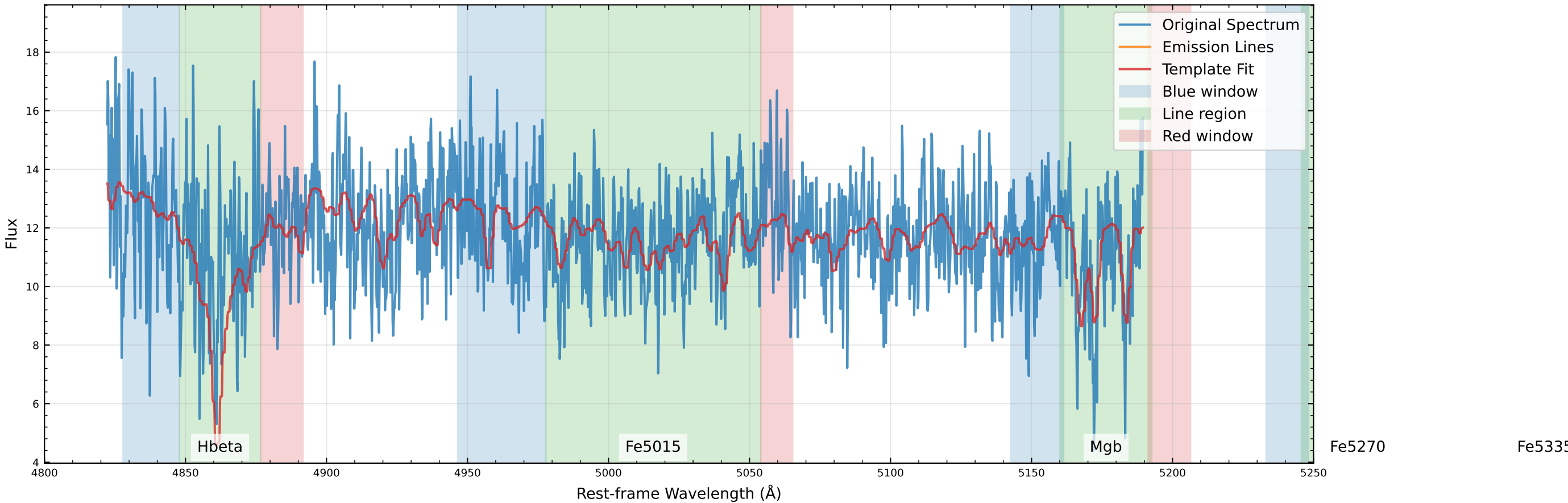
Original Data Comparison (v_star=-23.8 km/s, v_gas=22.4 km/s)
