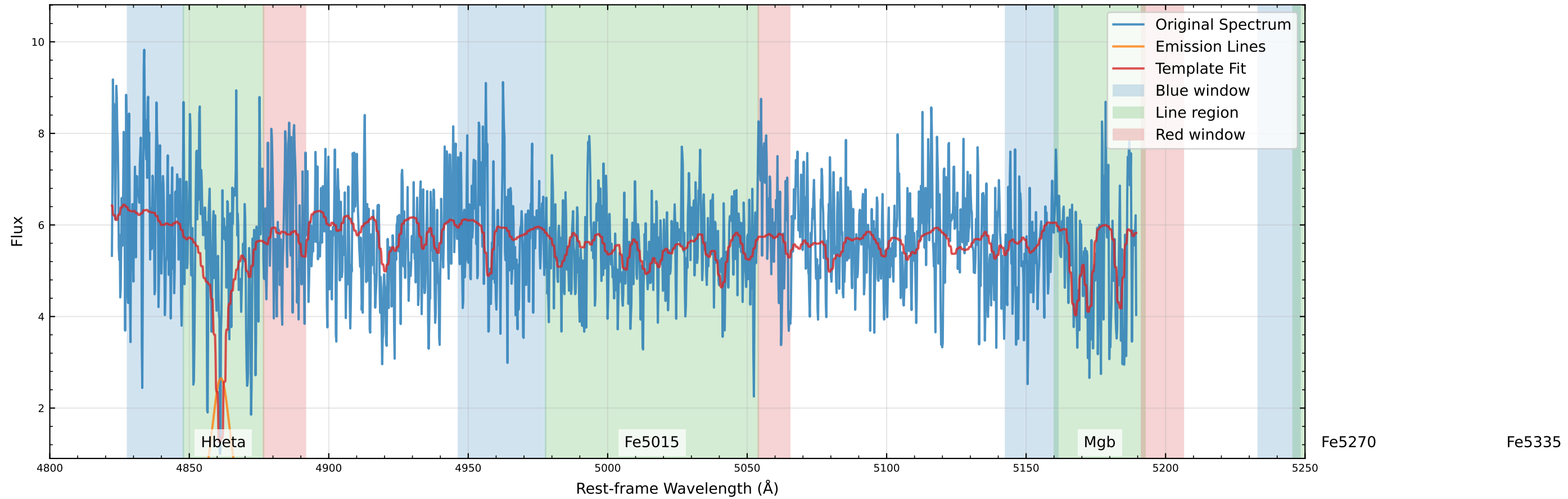
Original Data Comparison (v_star=5.5 km/s, v_gas=65.3 km/s)
