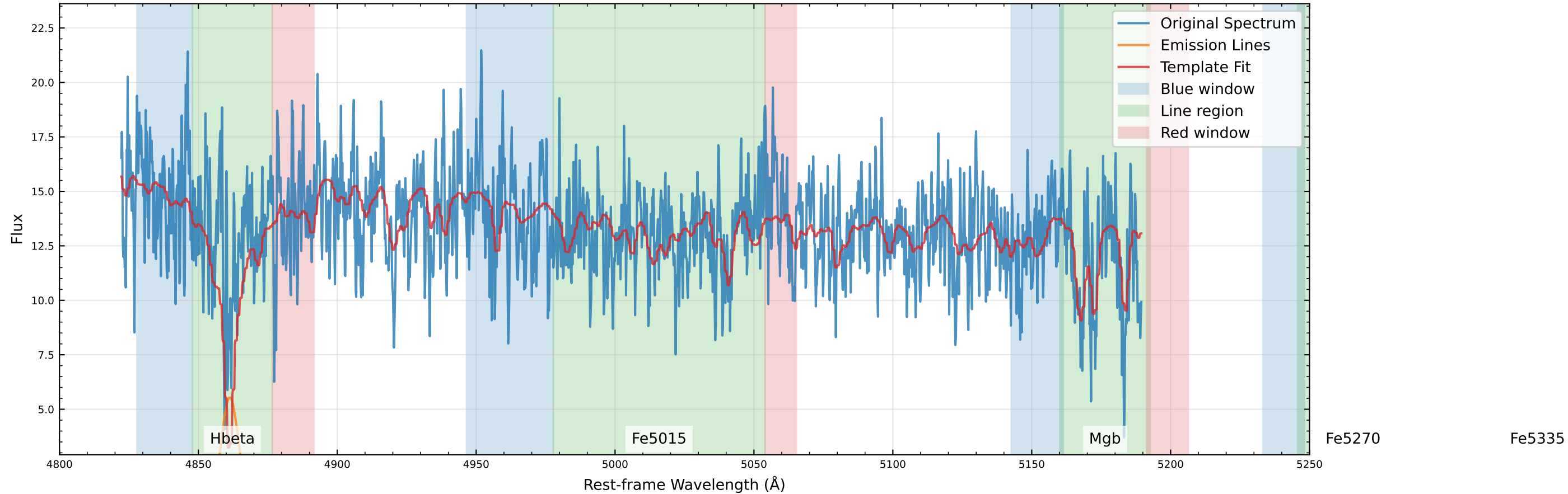
Original Data Comparison (v_star=-43.1 km/s, v_gas=-89.9 km/s)
