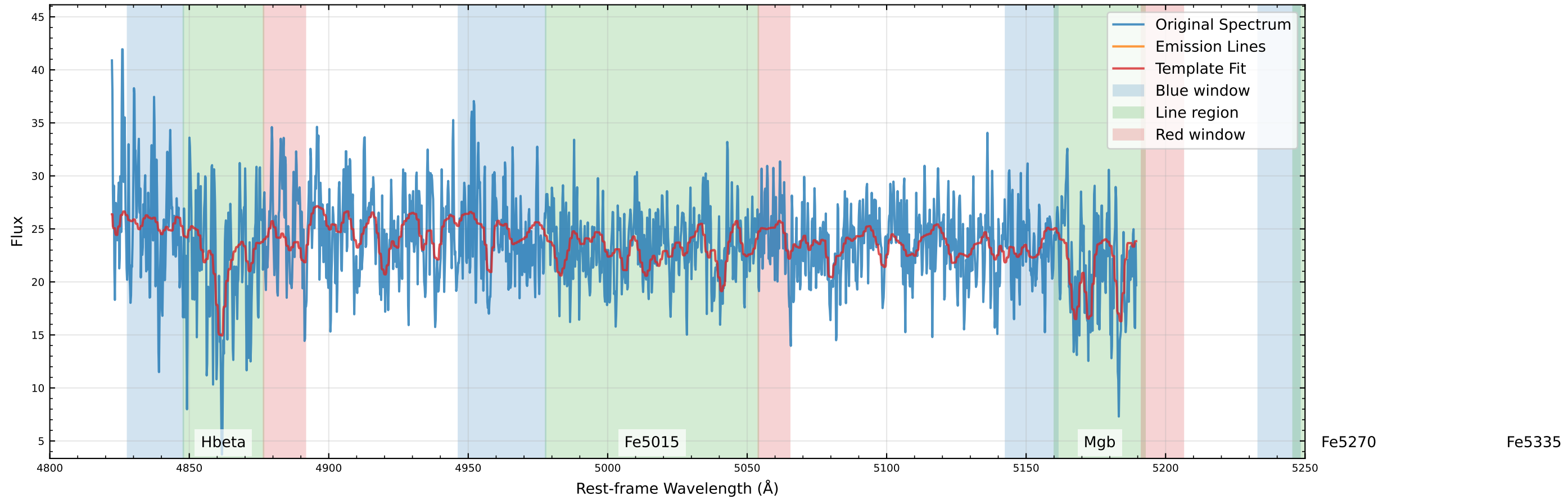
Original Data Comparison (v_star=13.7 km/s, v_gas=40.7 km/s)
