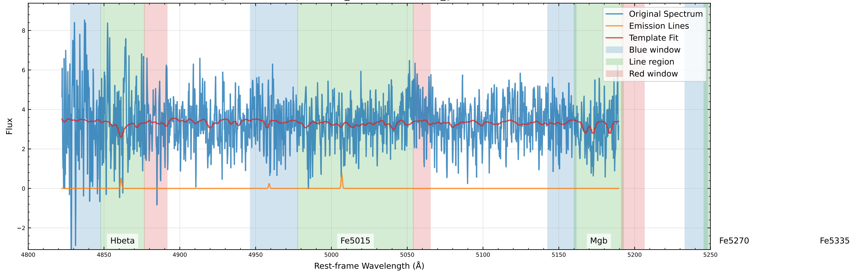
Original Data Comparison (v_star=-89.7 km/s, v_gas=-119.8 km/s)
