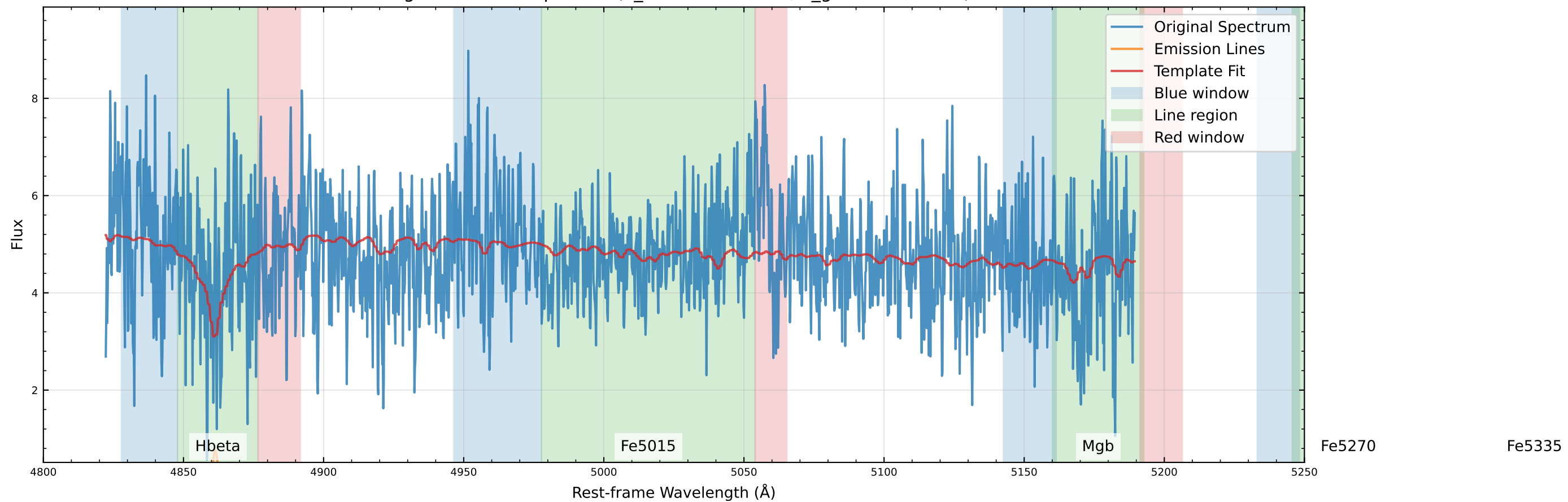
Original Data Comparison (v_star=-48.5 km/s, v_gas=-37.0 km/s)
