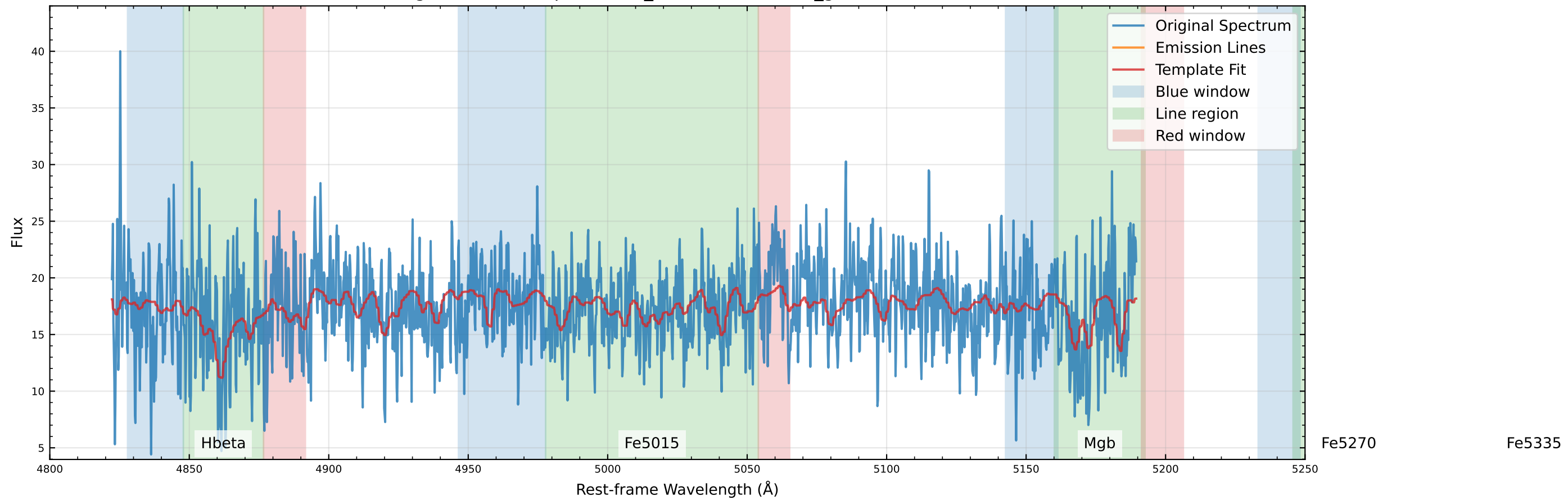
Original Data Comparison (v_star=15.0 km/s, v_gas=62.8 km/s)
