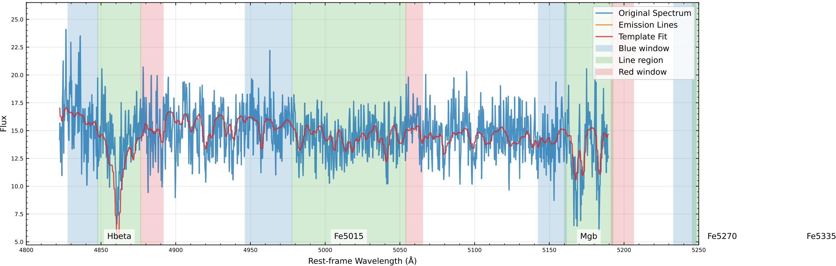
Original Data Comparison (v_star=-20.2 km/s, v_gas=-67.1 km/s)
