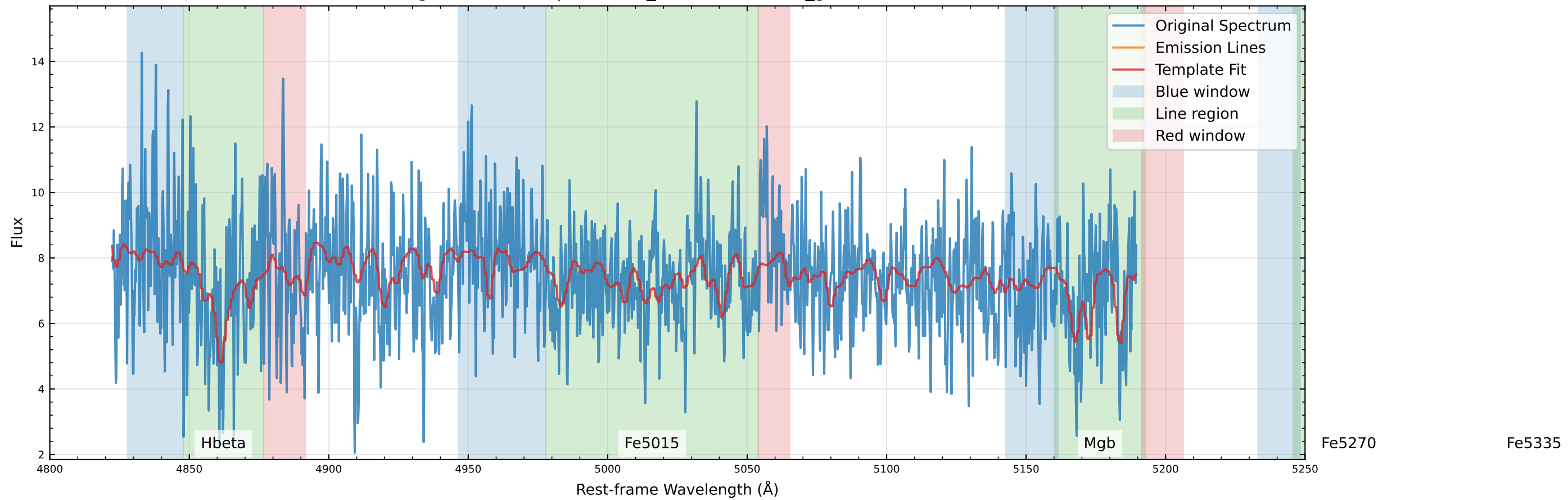
Original Data Comparison (v_star=3.1 km/s, v_gas=-81.7 km/s)
