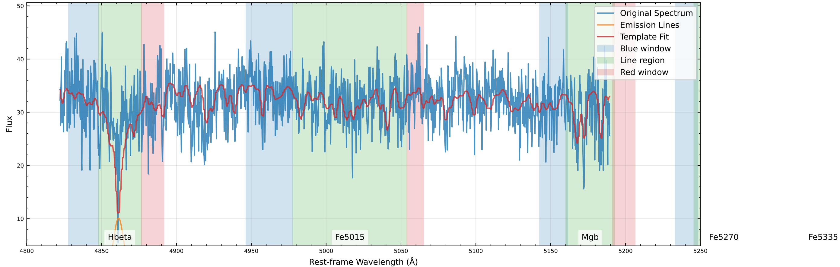
Original Data Comparison (v_star=-20.8 km/s, v_gas=7.6 km/s)
