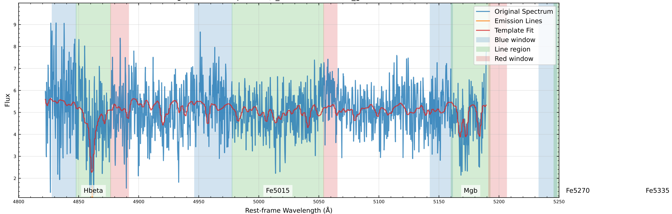
Original Data Comparison (v_star=-10.9 km/s, v_gas=2.5 km/s)
