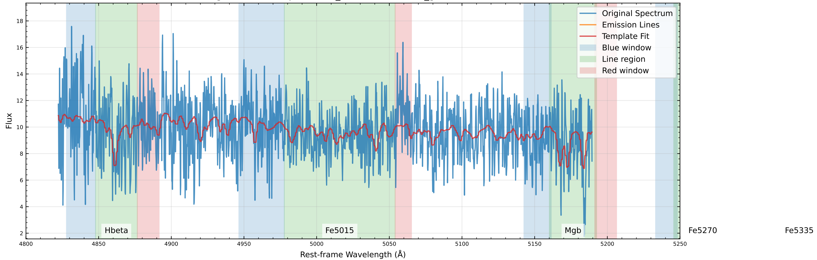
Original Data Comparison (v_star=40.9 km/s, v_gas=34.1 km/s)
