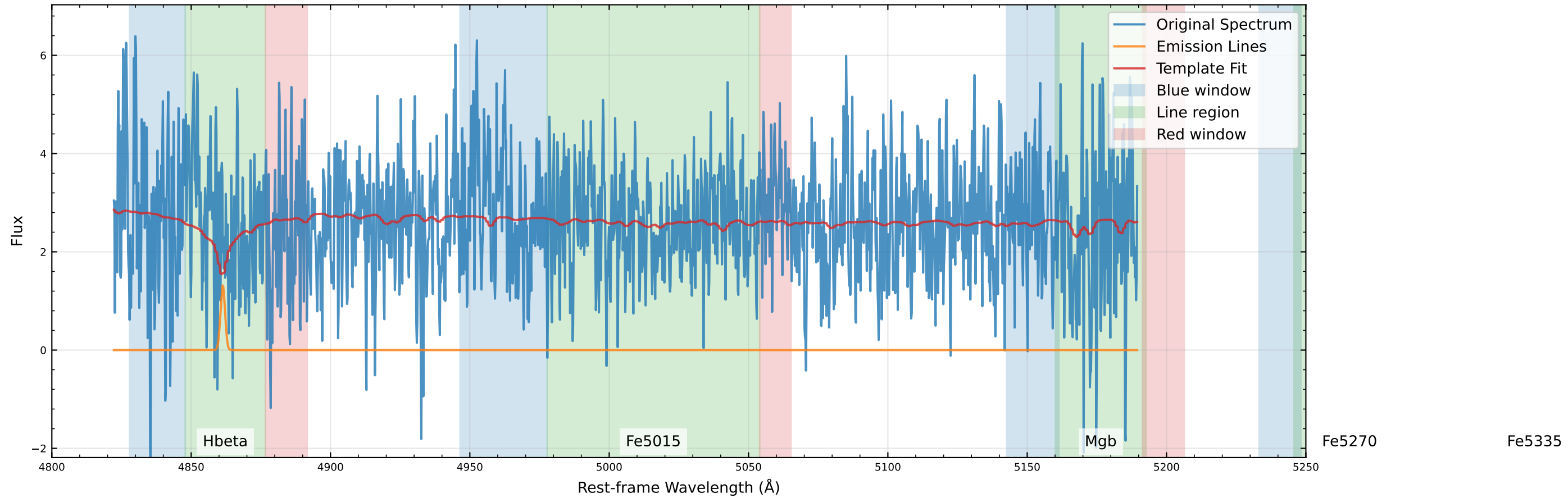
Original Data Comparison (v_star=-14.0 km/s, v_gas=-33.7 km/s)
