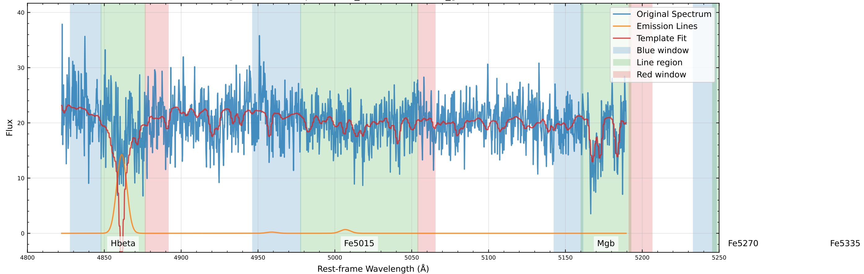
Original Data Comparison (v_star=-3.8 km/s, v_gas=-28.2 km/s)
