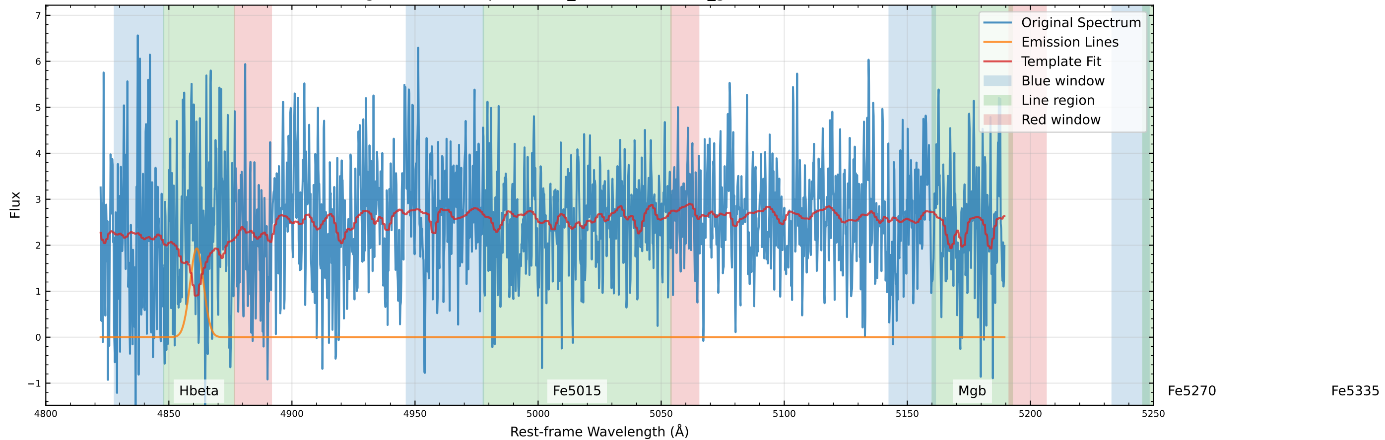
Original Data Comparison (v_star=8.3 km/s, v_gas=-129.9 km/s)
