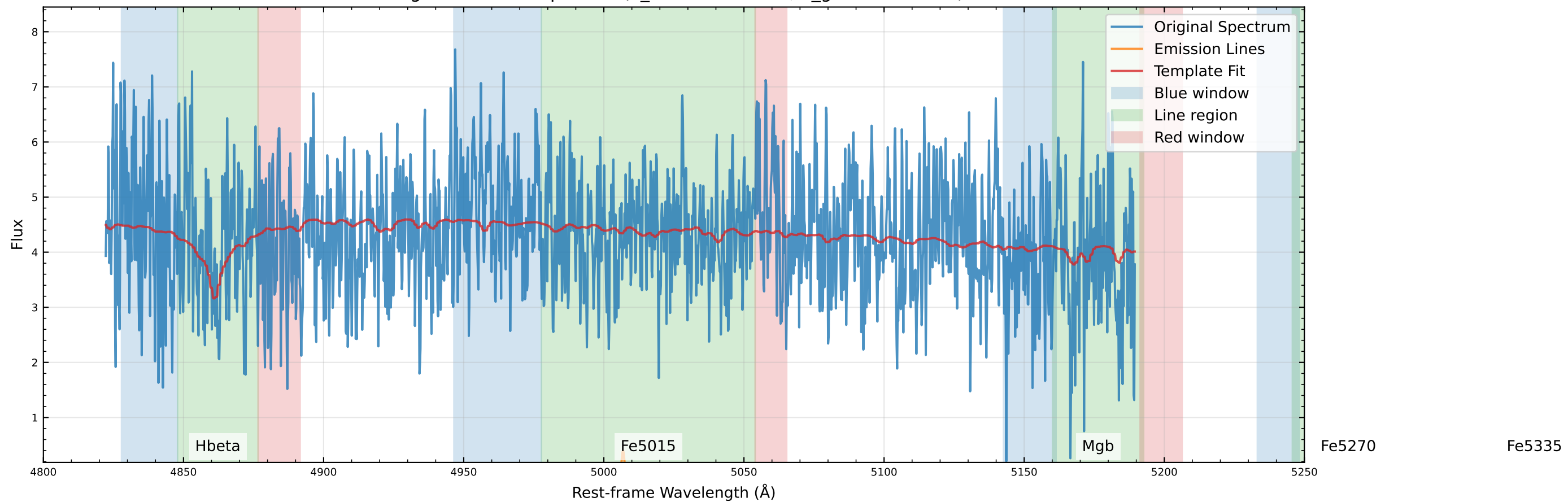
Original Data Comparison (v_star=16.8 km/s, v_gas=20.4 km/s)
