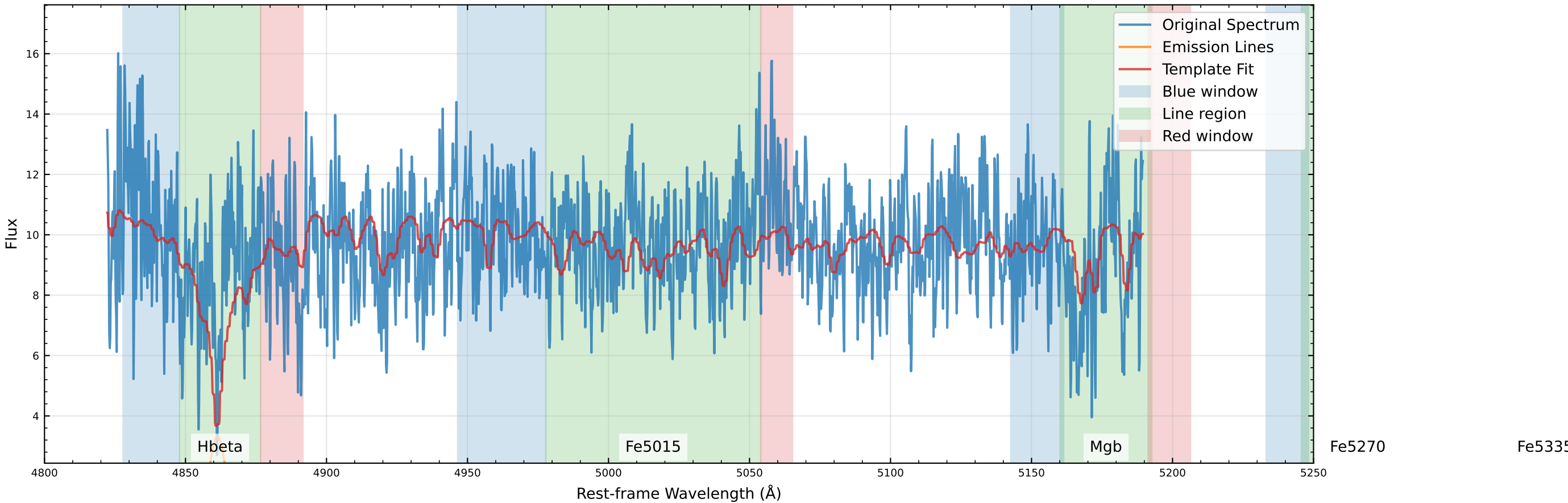
Original Data Comparison (v_star=-35.6 km/s, v_gas=87.5 km/s)
