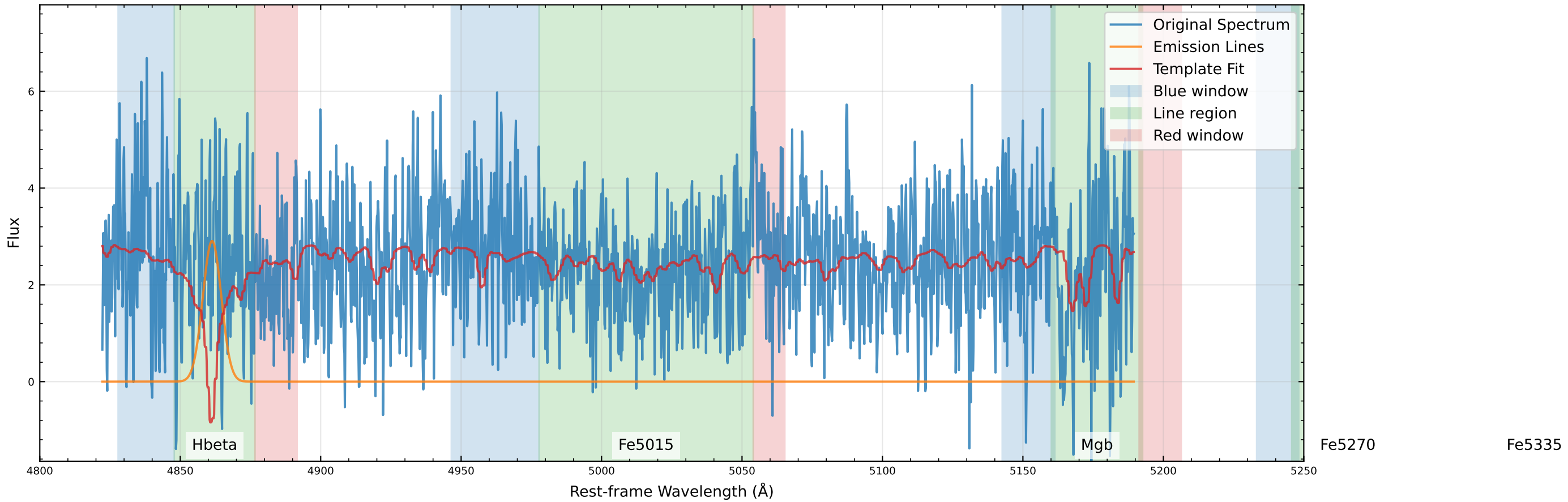
Original Data Comparison (v_star=-93.0 km/s, v_gas=-85.3 km/s)
