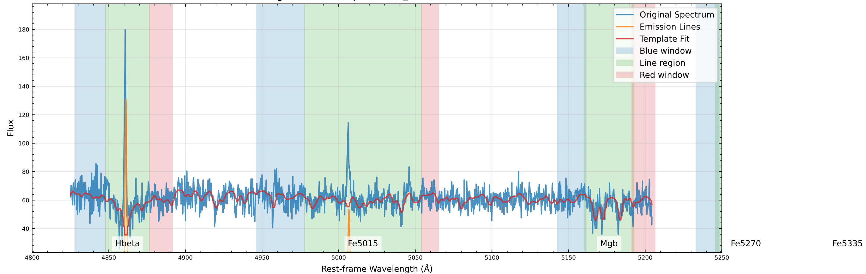
Original Data Comparison (v_star=-30.0 km/s)
