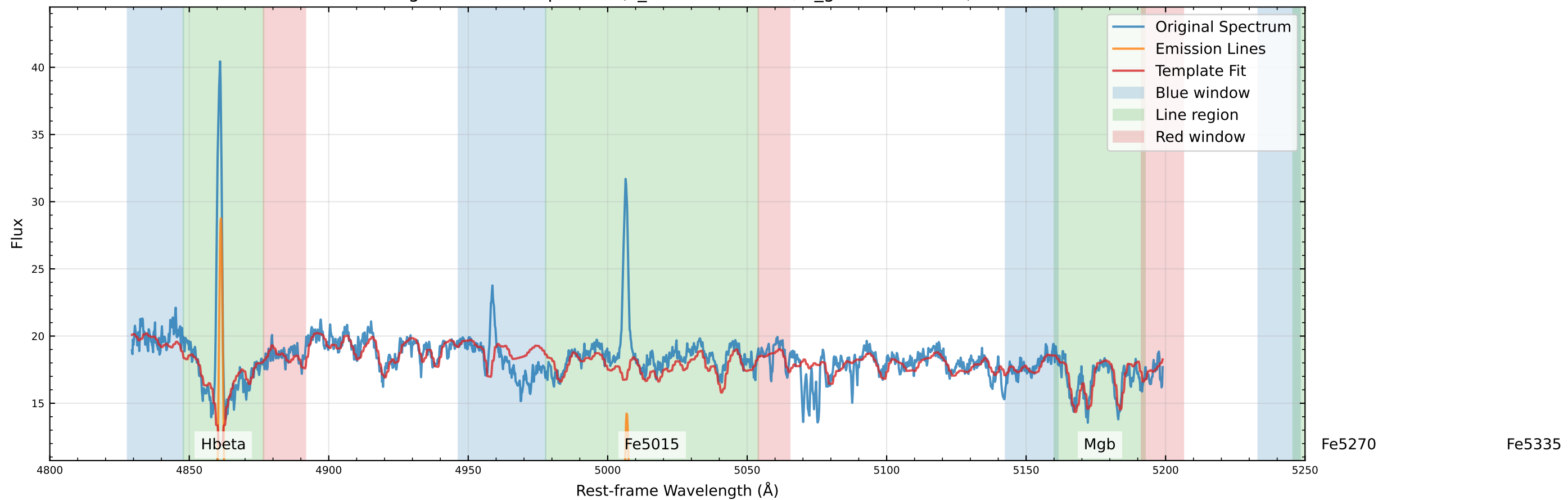
Original Data Comparison (v_star=-41.7 km/s, v_gas=-32.1 km/s)
