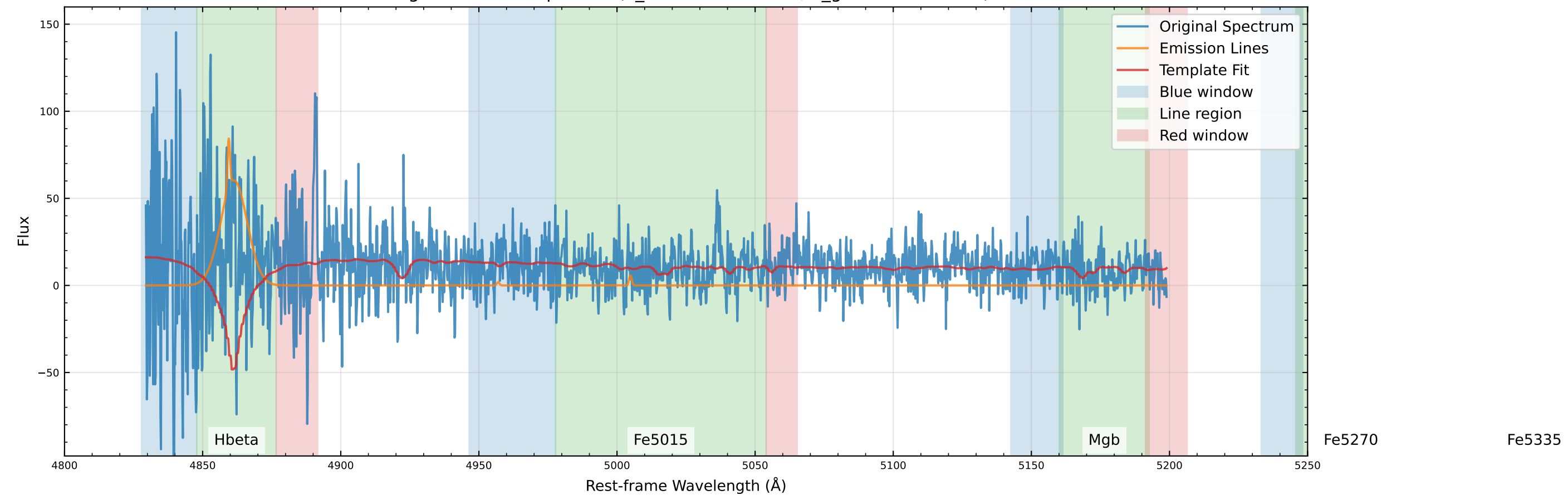
Original Data Comparison (v_star=-416.9 km/s, v_gas=-253.3 km/s)
