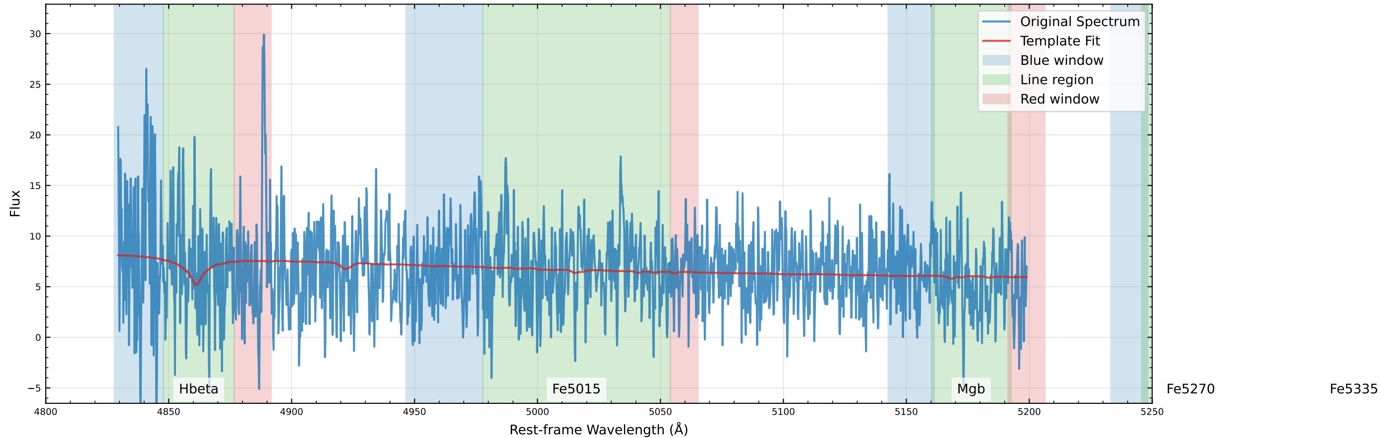
Original Data Comparison (v_star=78.5 km/s)
