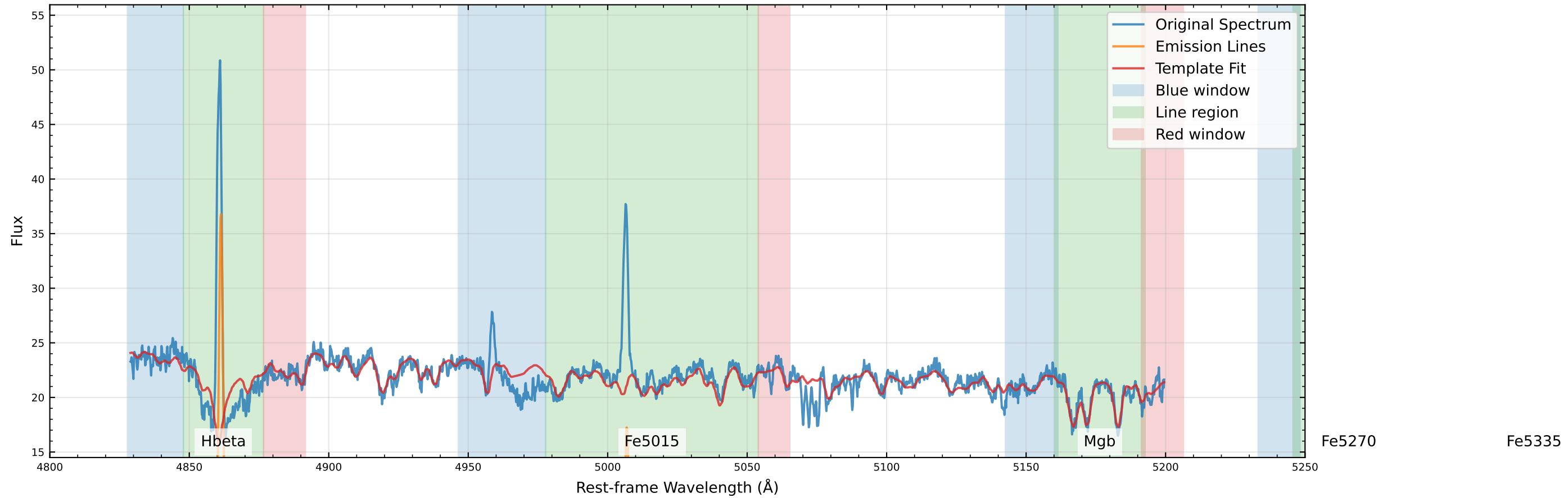
Original Data Comparison (v_star=-41.9 km/s, v_gas=-35.1 km/s)
