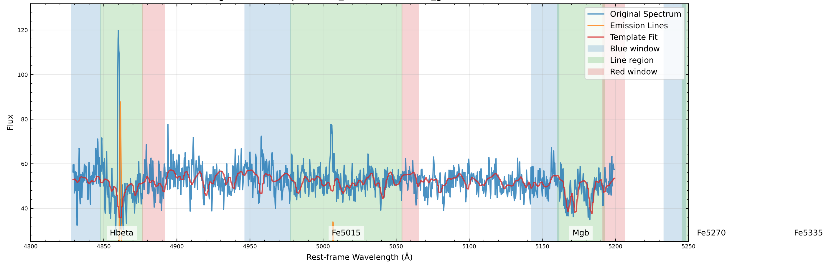
Original Data Comparison (v_star=-75.4 km/s, v_gas=-75.0 km/s)
