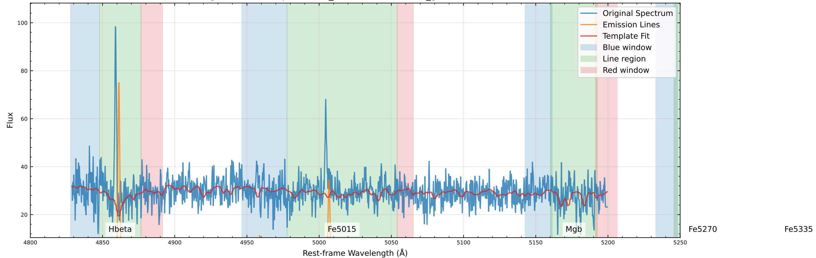
Original Data Comparison (v_star=-135.1 km/s, v_gas=-138.4 km/s)
