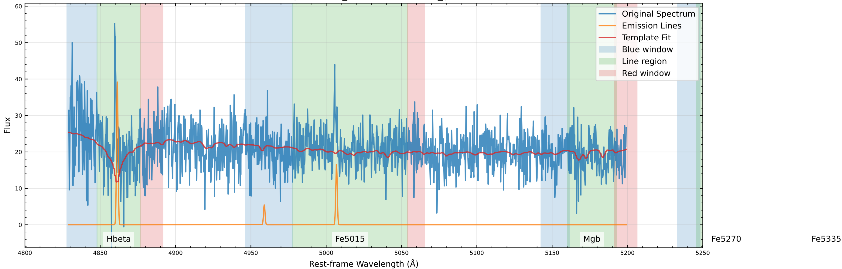
Original Data Comparison (v_star=-44.1 km/s, v_gas=-83.4 km/s)
