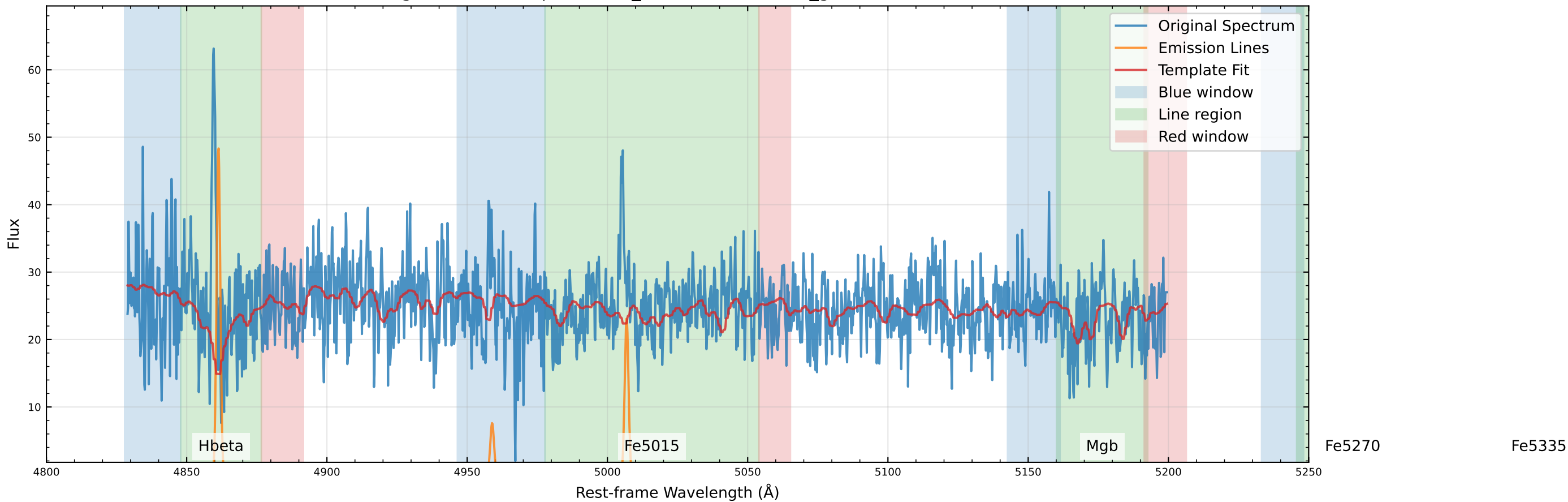
Original Data Comparison (v_star=-80.9 km/s, v_gas=-100.3 km/s)
