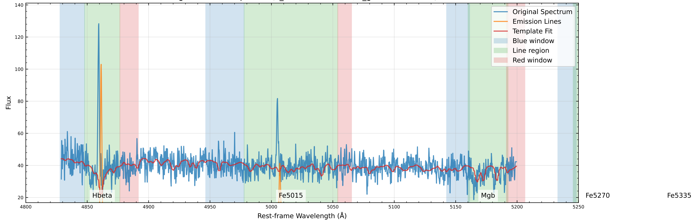
Original Data Comparison (v_star=-114.1 km/s, v_gas=-124.2 km/s)
