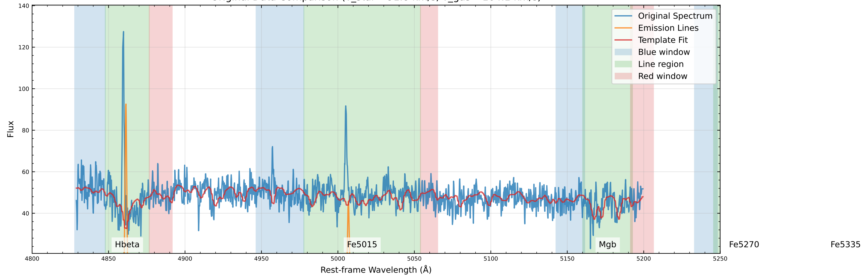
Original Data Comparison (v_star=-91.8 km/s, v_gas=-104.1 km/s)
