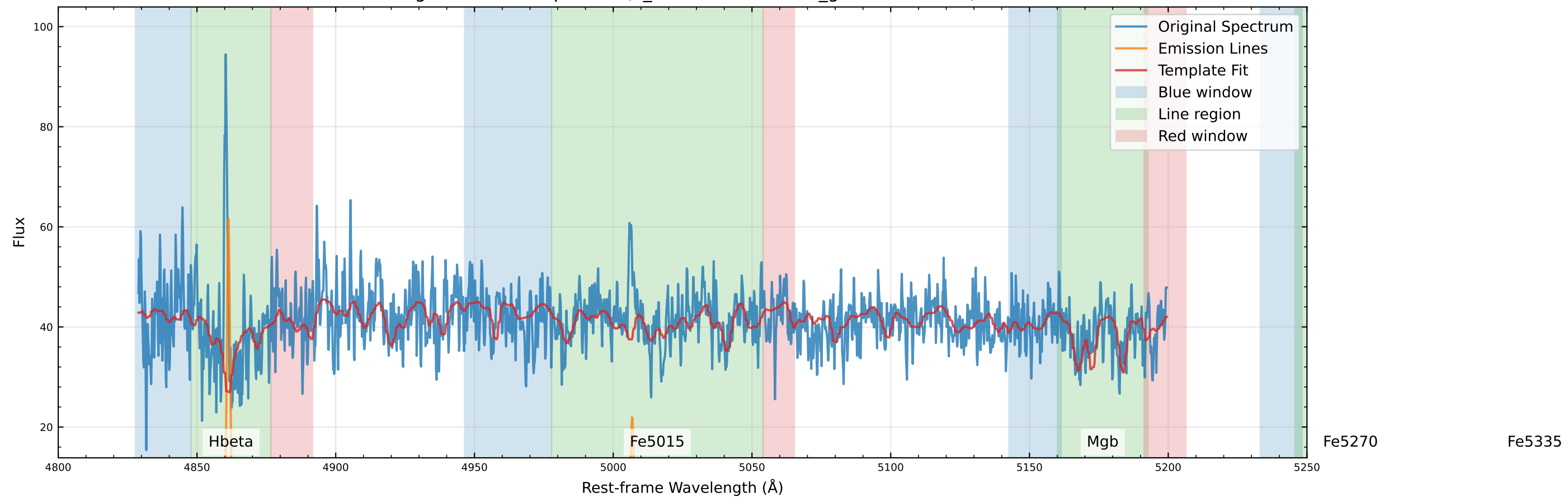
Original Data Comparison (v_star=-50.9 km/s, v_gas=-56.4 km/s)
