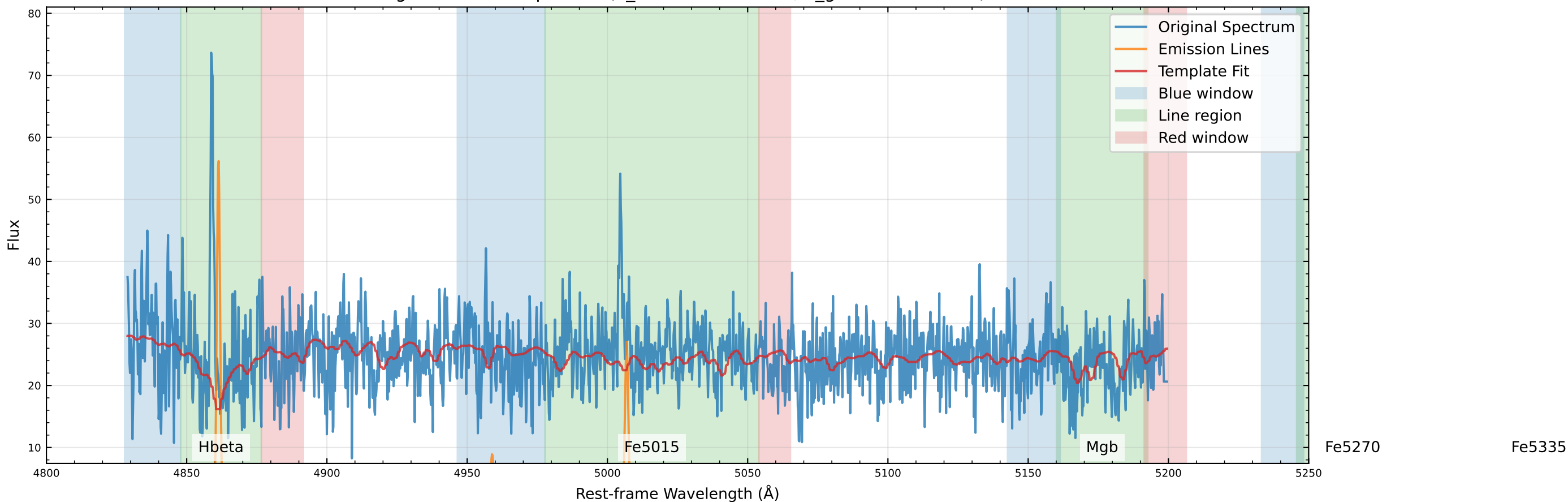
Original Data Comparison (v_star=-135.0 km/s, v_gas=-140.9 km/s)
