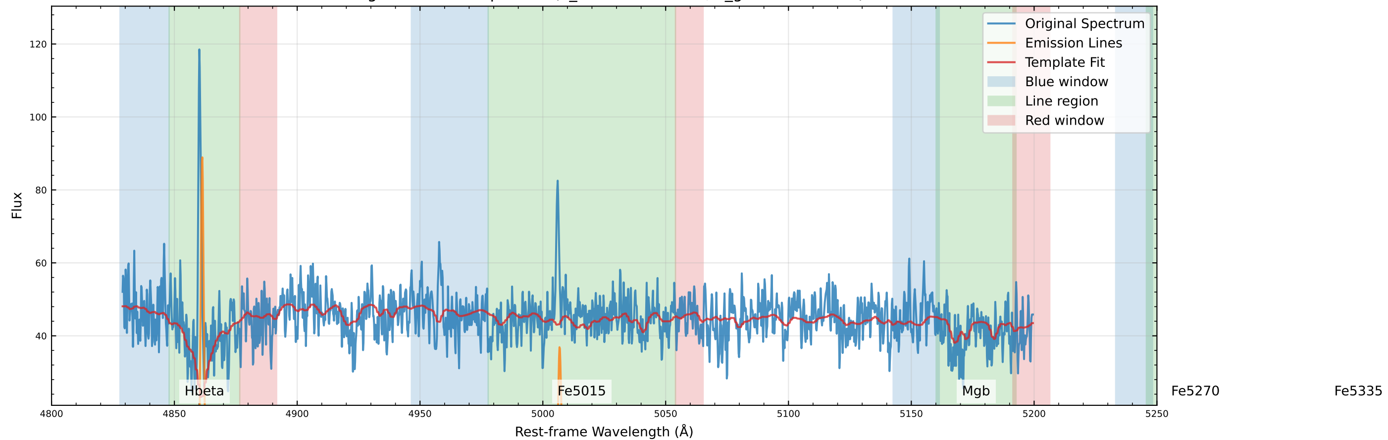
Original Data Comparison (v_star=-55.6 km/s, v_gas=-60.8 km/s)
