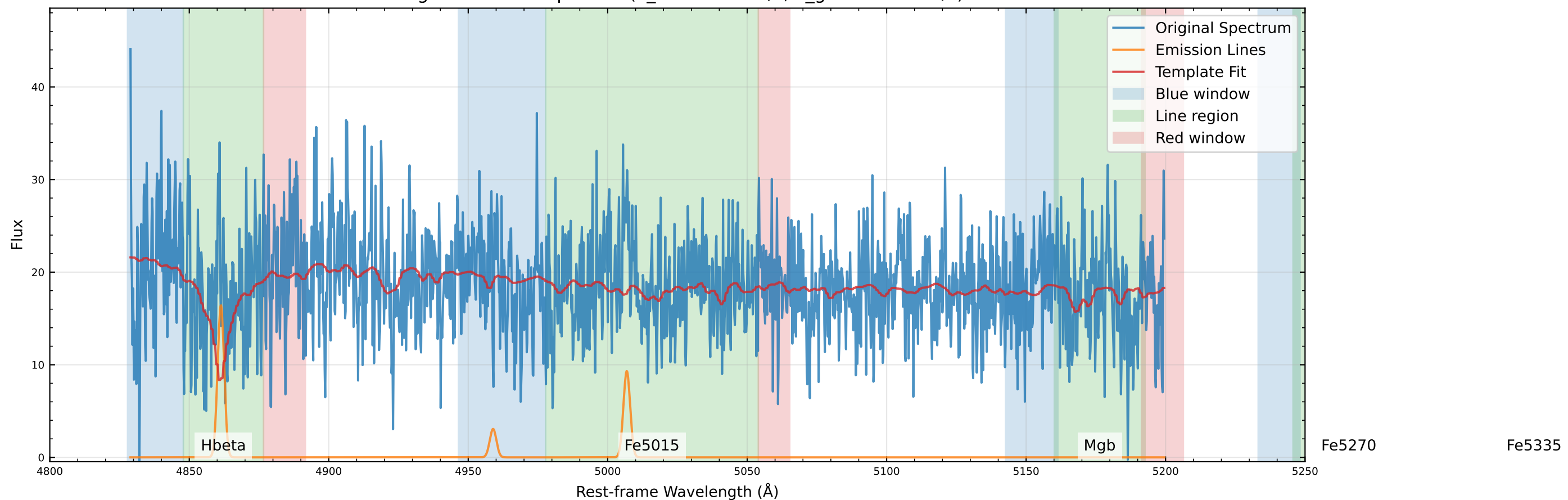
Original Data Comparison (v_star=3.6 km/s, v_gas=-26.9 km/s)
