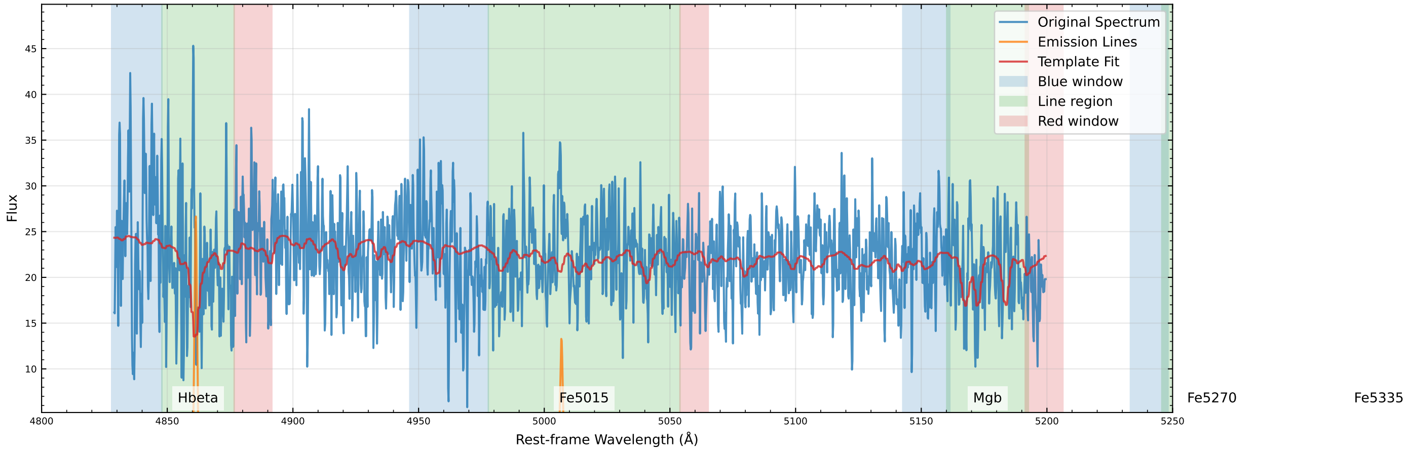
Original Data Comparison (v_star=-50.7 km/s, v_gas=-59.8 km/s)
