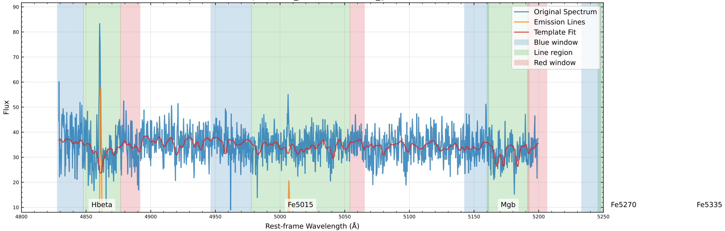
Original Data Comparison (v_star=-56.8 km/s, v_gas=-46.0 km/s)
