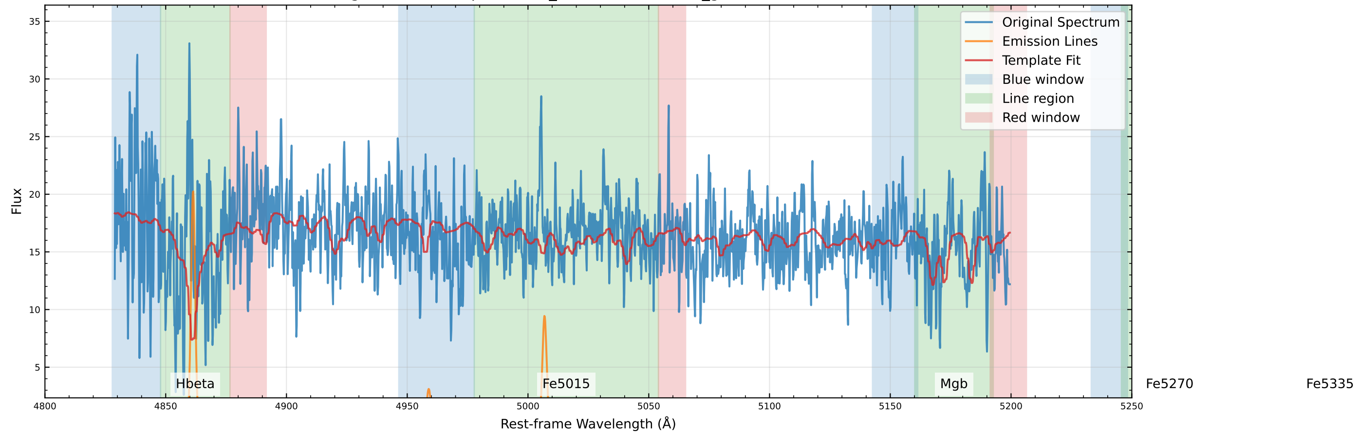
Original Data Comparison (v_star=-89.5 km/s, v_gas=-100.5 km/s)
