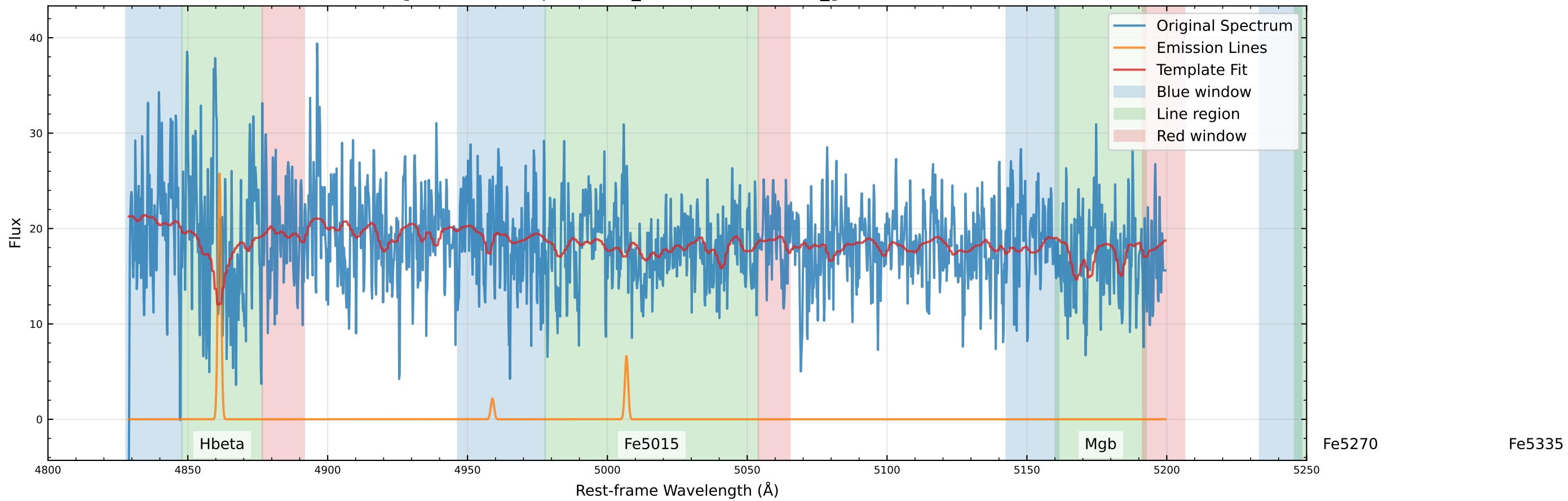
Original Data Comparison ( v_{\text{star}}=-101.2 km/s, v_{\text{gas}}=-98.6 km/s)
