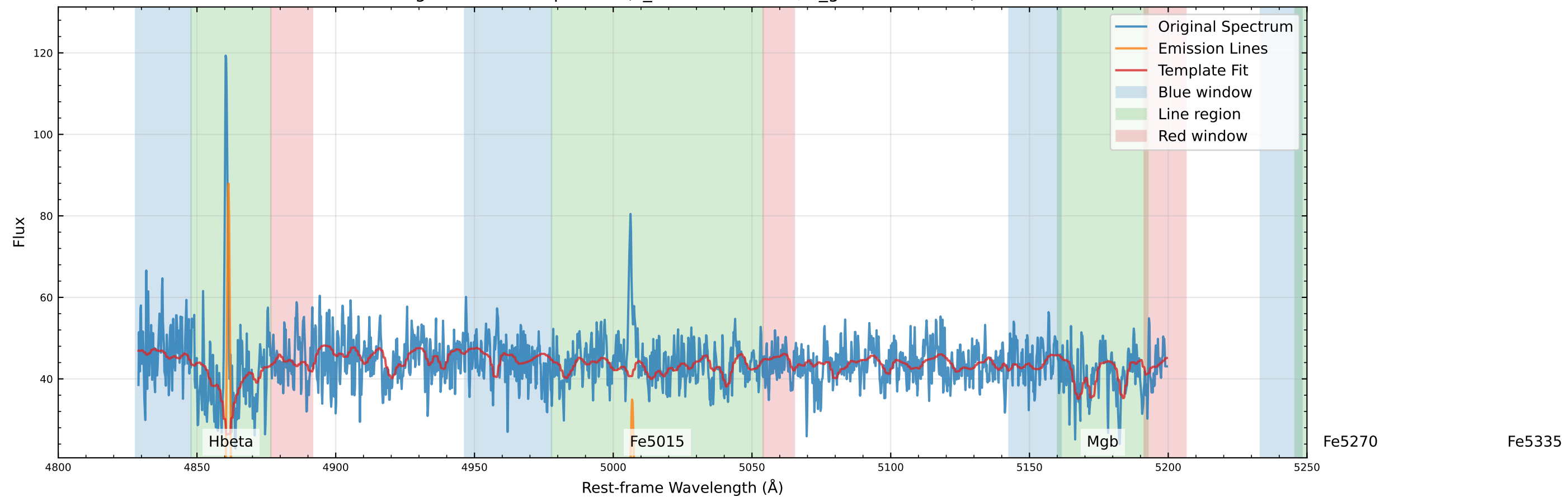
Original Data Comparison (v_star=-69.8 km/s, v_gas=-49.1 km/s)
