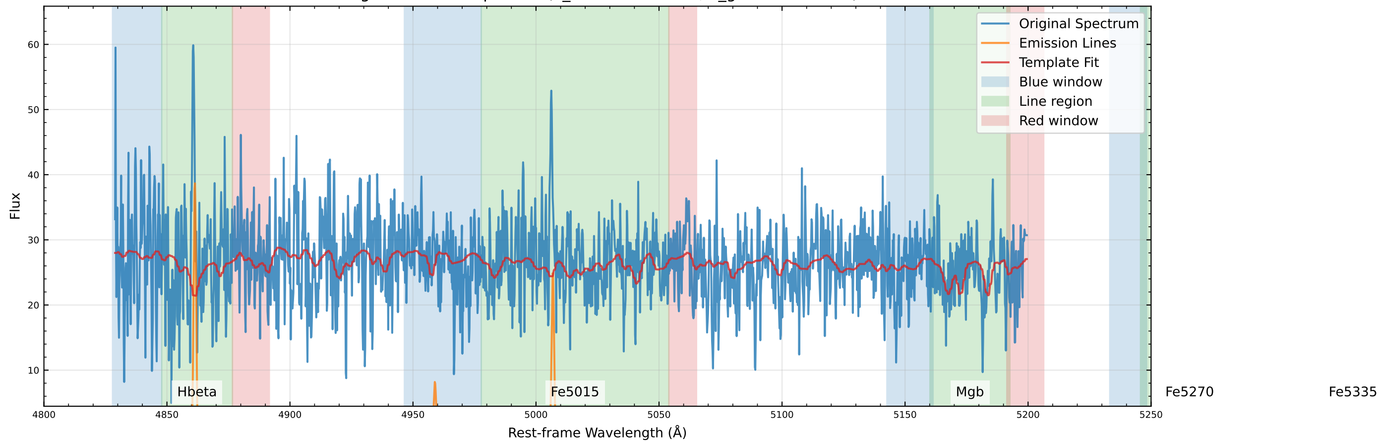
Original Data Comparison ( v_{\text{star}}=-52.8 km/s, v_{\text{gas}}=-39.1 km/s)
