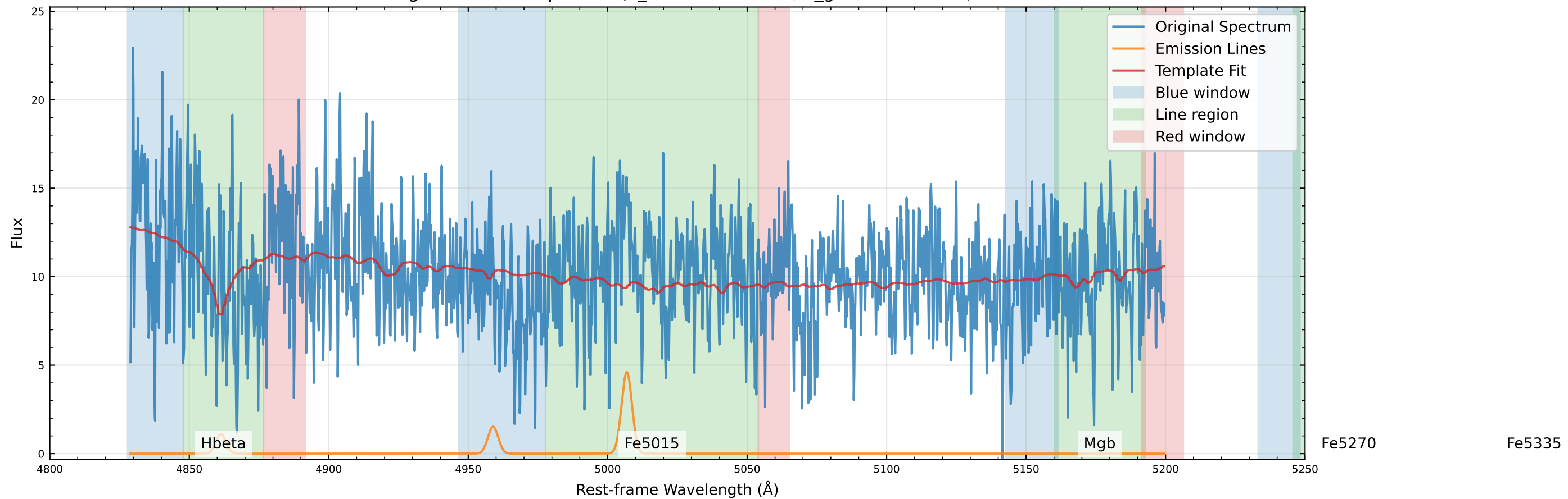
Original Data Comparison (v_star=-10.3 km/s, v_gas=-57.9 km/s)
