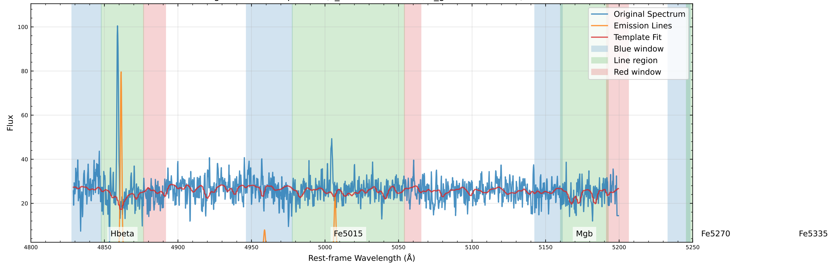
Original Data Comparison (v_star=-138.8 km/s, v_gas=-141.8 km/s)
