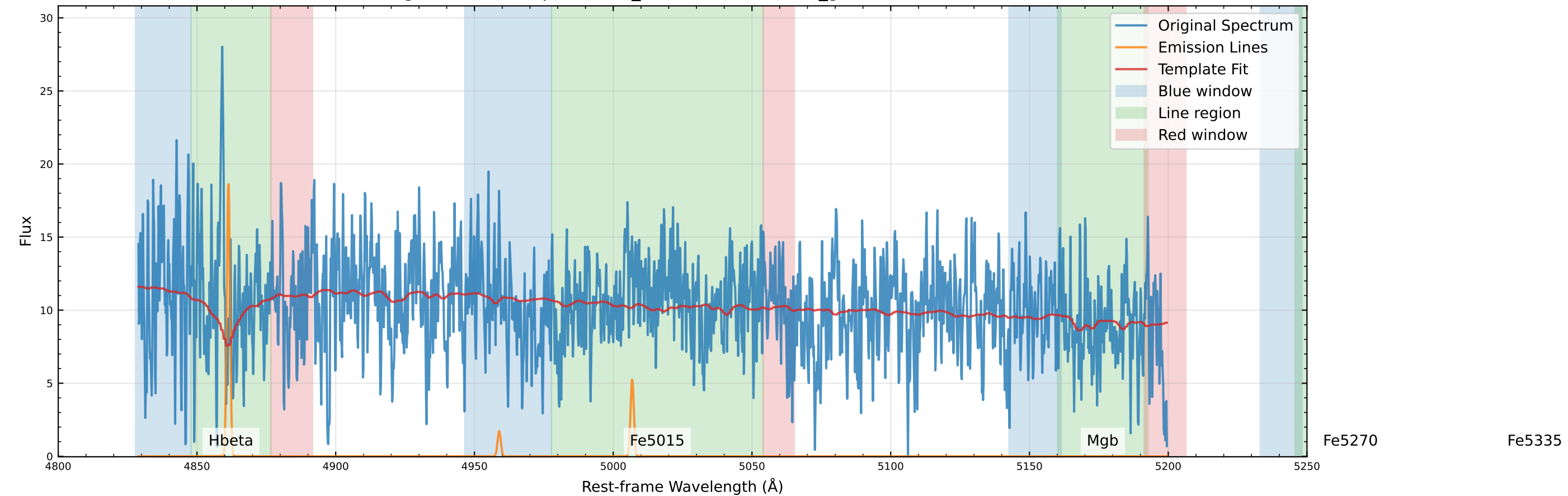
Original Data Comparison (v_star=-151.1 km/s, v_gas=-142.3 km/s)
