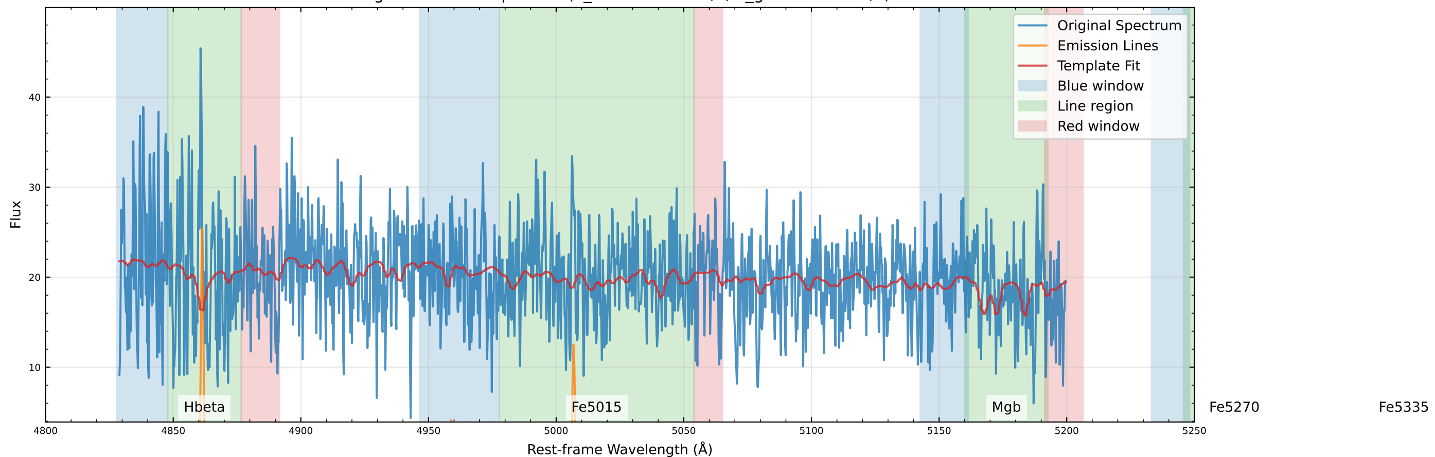
Original Data Comparison (v_star=-21.0 km/s, v_gas=-29.2 km/s)
