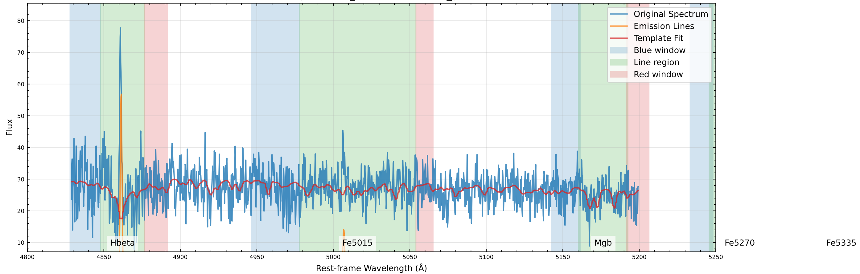
Original Data Comparison ( v_{\text{star}}=-47.9 km/s, v_{\text{gas}}=-30.2 km/s)
