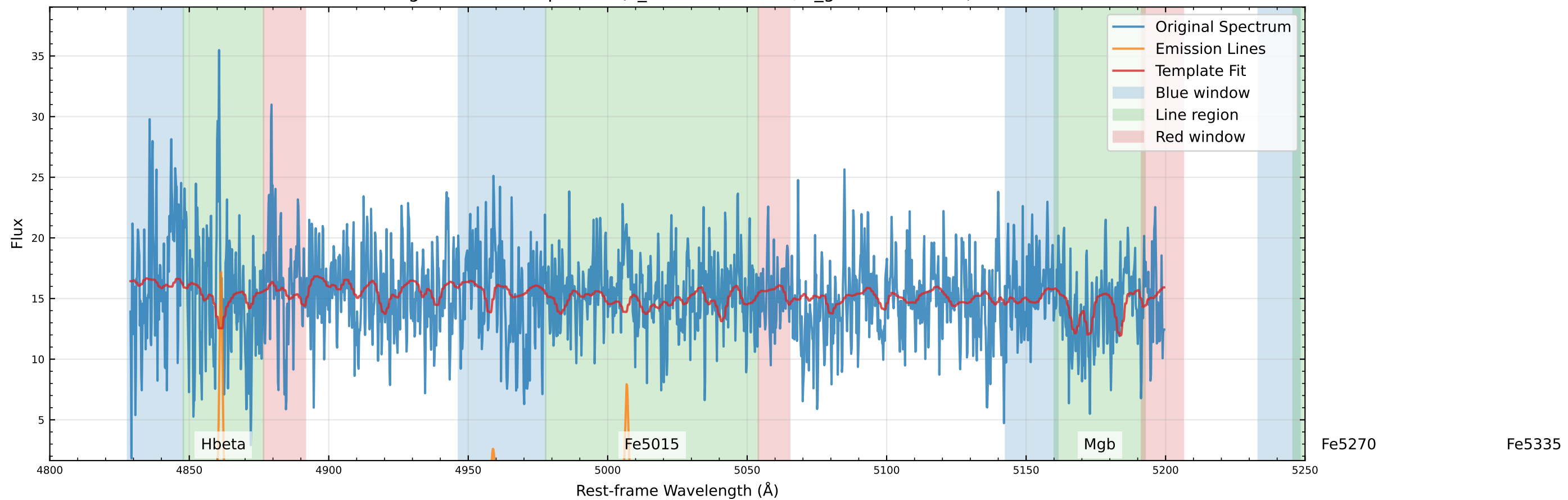
Original Data Comparison (v_star=-64.9 km/s, v_gas=-54.0 km/s)
