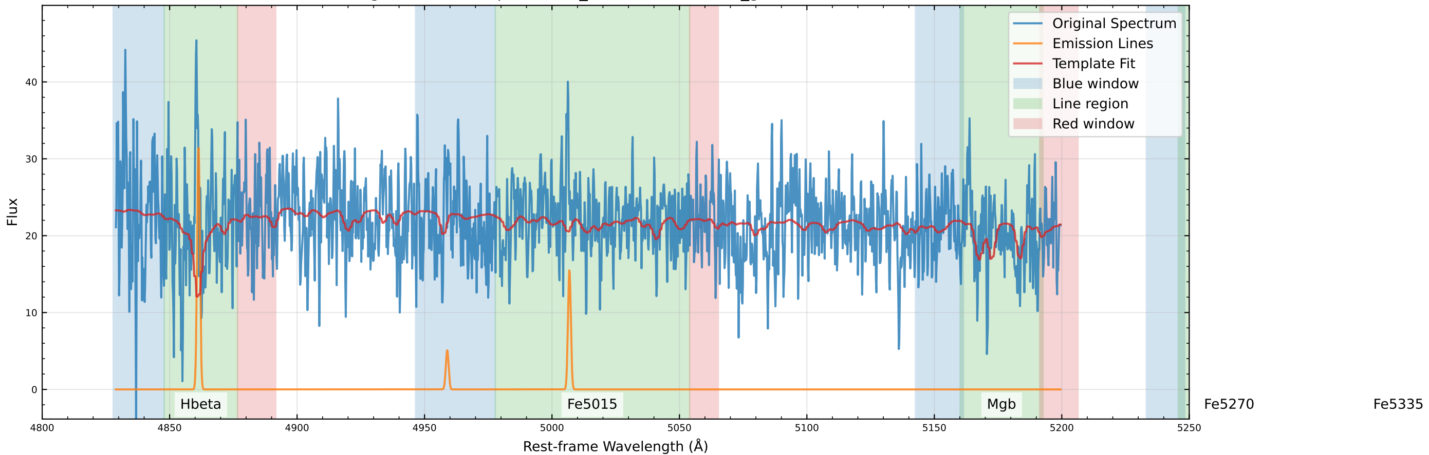
Original Data Comparison (v_star=-52.5 km/s, v_gas=-47.1 km/s)
