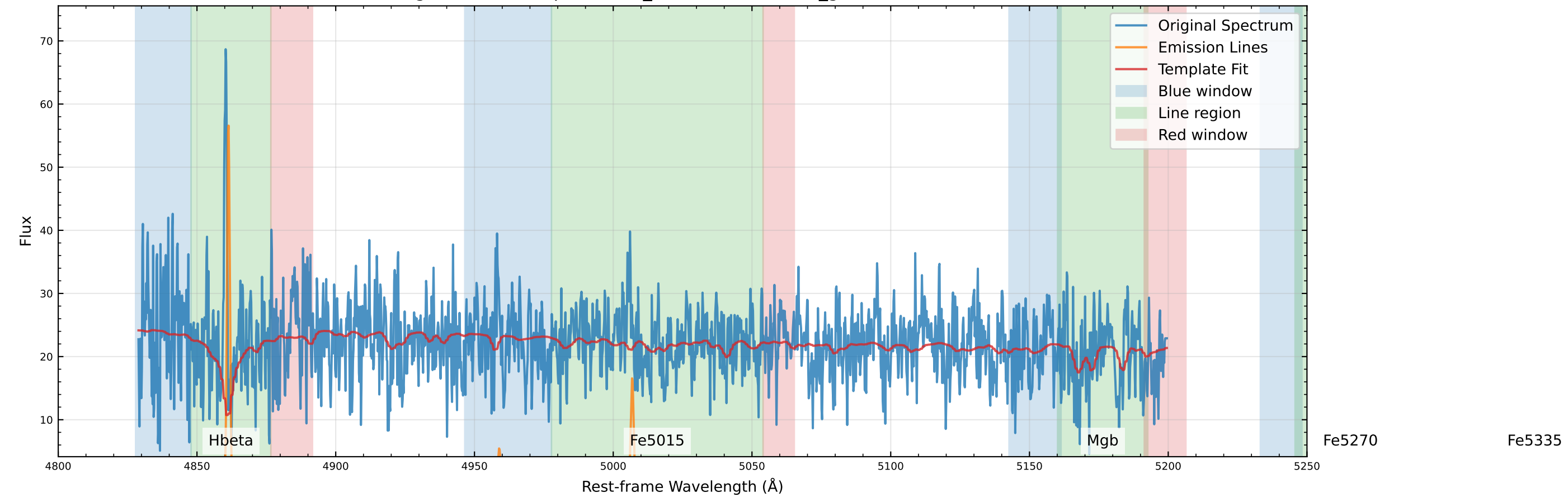
Original Data Comparison (v_star=-84.5 km/s, v_gas=-65.7 km/s)
