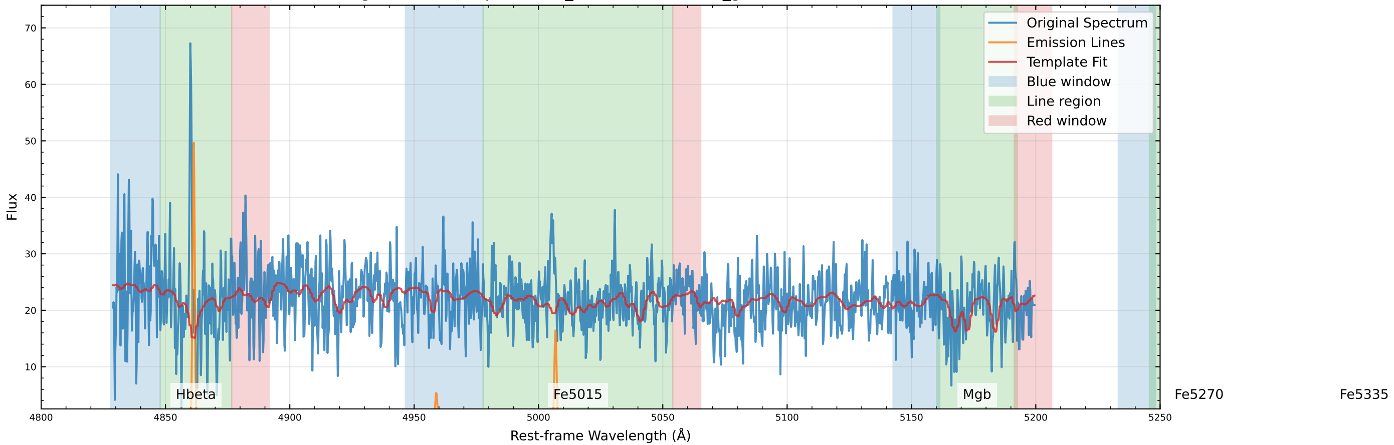
Original Data Comparison (v_star=-92.5 km/s, v_gas=-76.6 km/s)
