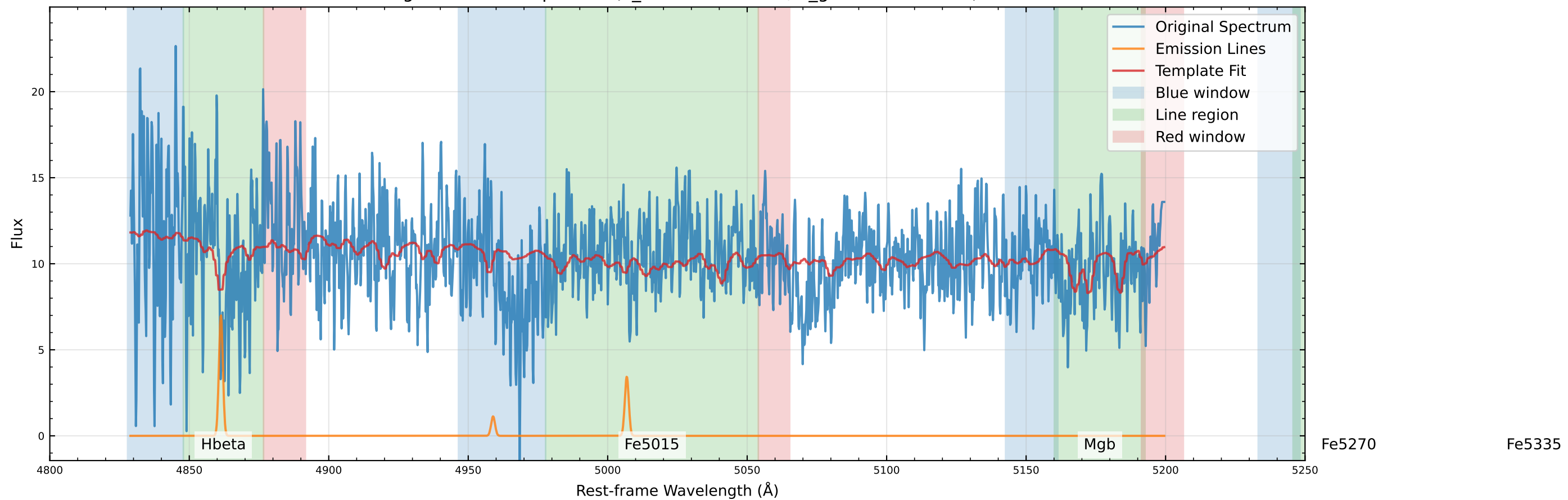
Original Data Comparison (v_star=-98.6 km/s, v_gas=-111.5 km/s)
